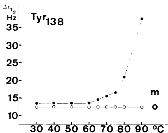
Fig.2. Temperature-dependent line broadening of the 2,6-proton doublet of Tyr 138 . The linewidth of the resonances were measured (in Hz) at half height and plotted vs temperature. ('m') doublet of the protons meta to the hydroxyl group = 2,6-doublet; ('o') doublet of the protons ortho to the hydroxyl group = 3,5-doublet.
